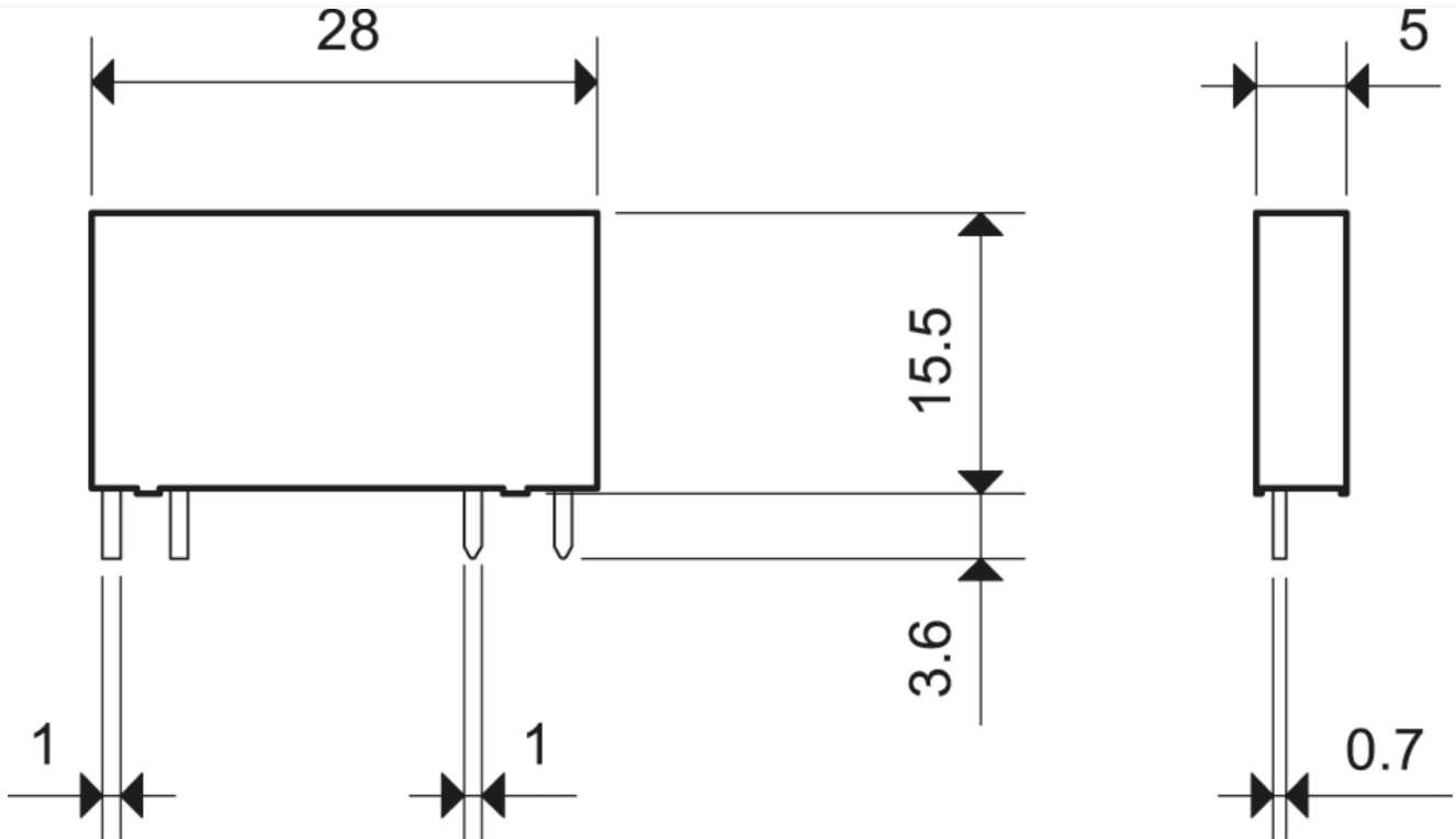
Dimension Diagram
