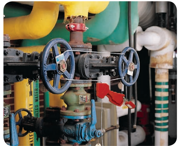
The original Cable Lockout device enables you to lock out several disconnects in various energy distribution centres simultaneously.
