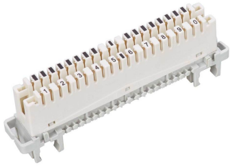
LSA-PLUS® Disconnection Module, cat 3, 2/10, PROFIL mounting
