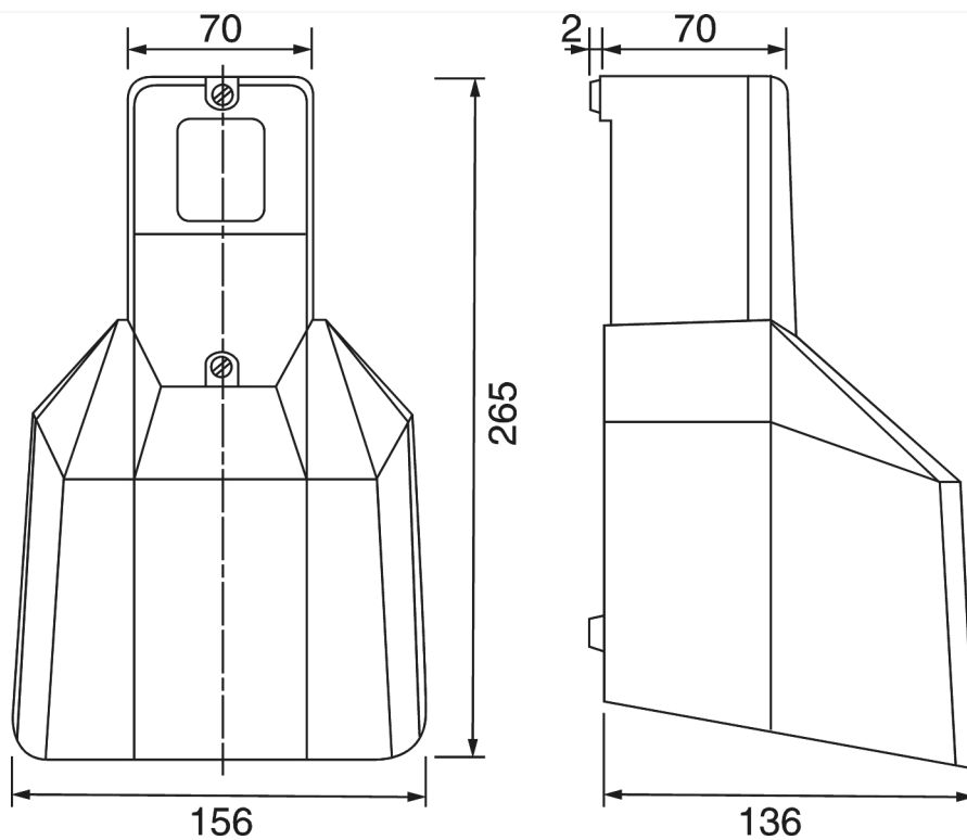
Dimension Diagram
