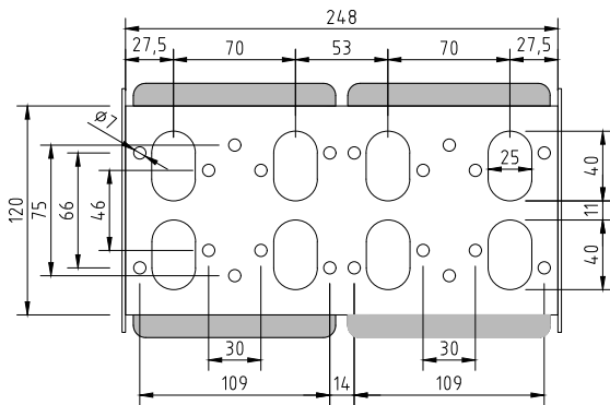
AFB20/2 CABLE ENTRY DETAILS
