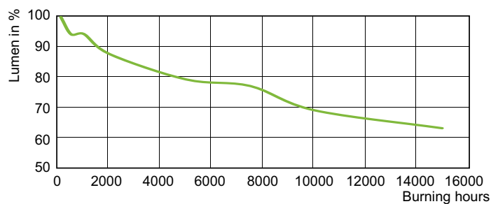
LDLM_MH_0008-Lumen maintenance diagram
