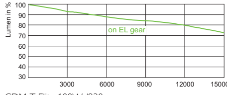
CDM-T Elite 100W /930
