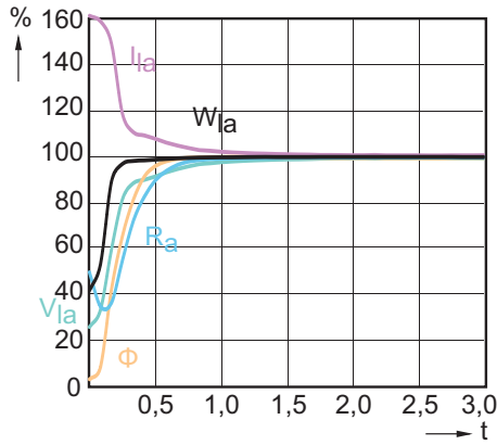
CDM-TC Elite 35W /842, /930, /942
