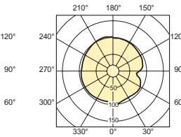
CDM-TC Elite 35W /842, /930, /942
