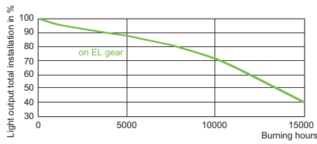
CDM-TC Elite 35W /930
