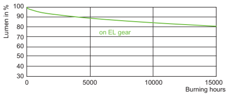
CDM-TC Elite 35W /842, /942
