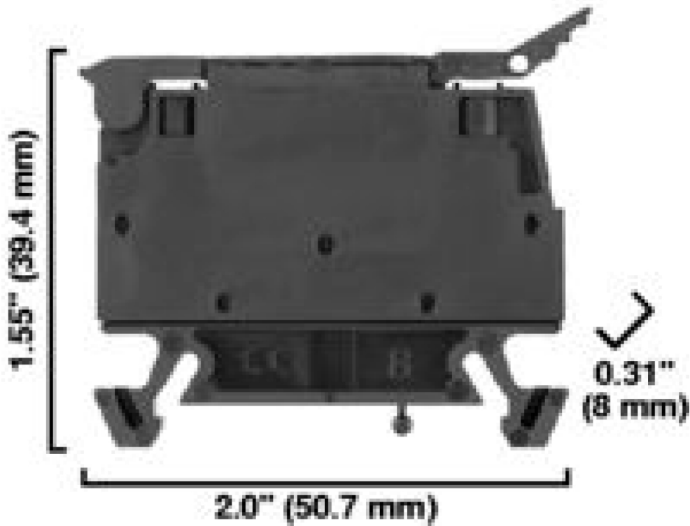
Dimension Diagram
