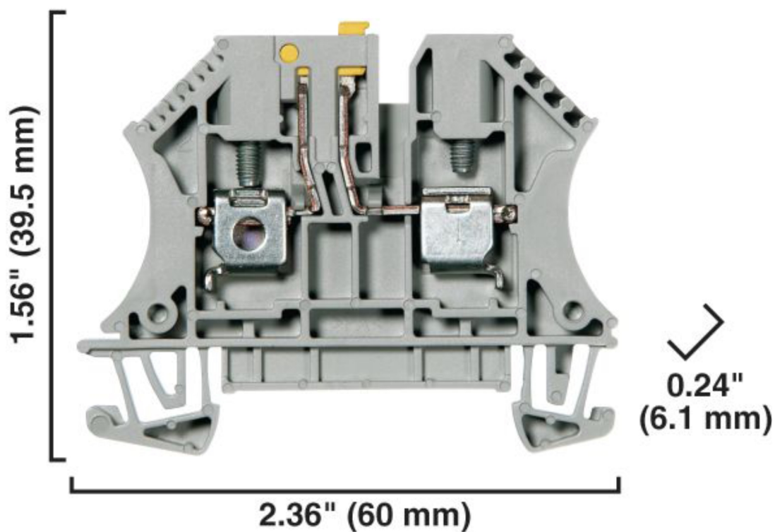
Dimension Diagram
