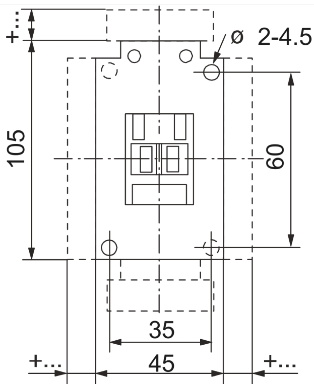
Dimension Diagram
