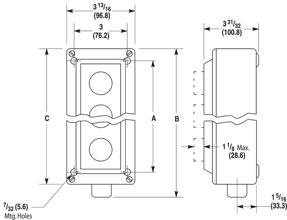
Type 4/4X/13 Rosite Glass Polyester Watertight, Oiltight, Corrosion Resistant Enclosure Dimension Diagram
