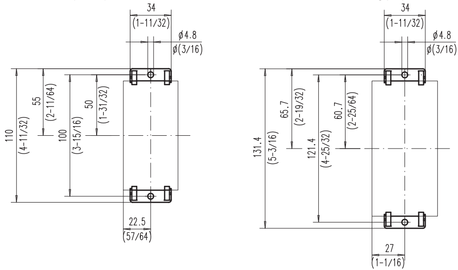
Screw Adapter 140M-C-N45 for 140M-C2/D8 and 140M-F8
