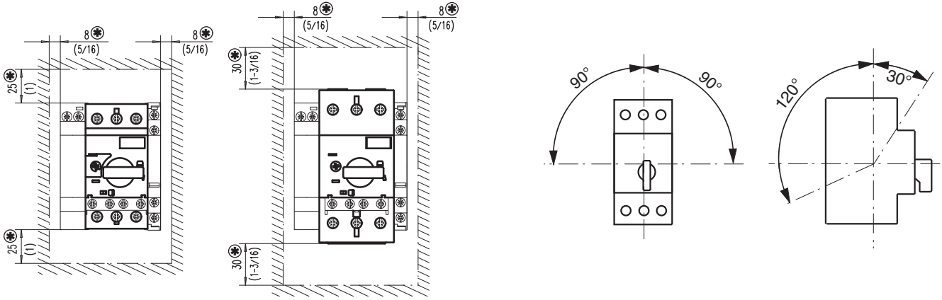
Mounting position/safety clearance of Cat. No. 140M-C..., 140M-D..., 140M-F...
