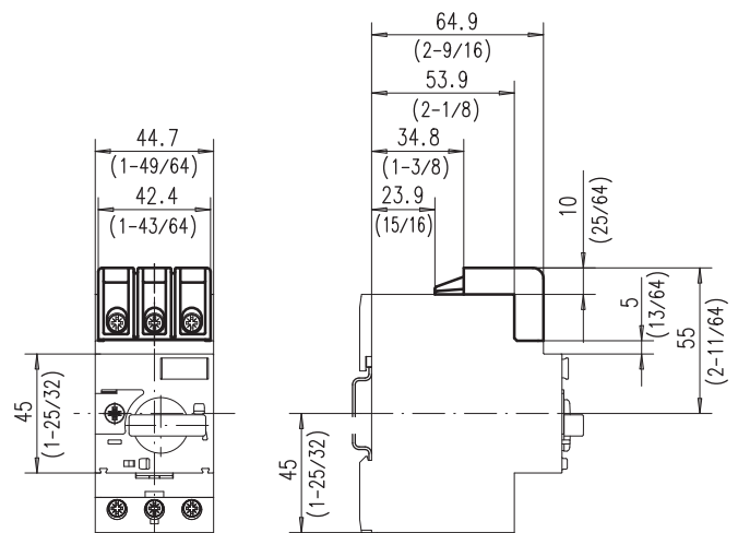
Cat. No. 140M-C-TE1 Type E adapter on Cat. No. 140M-D8E...
