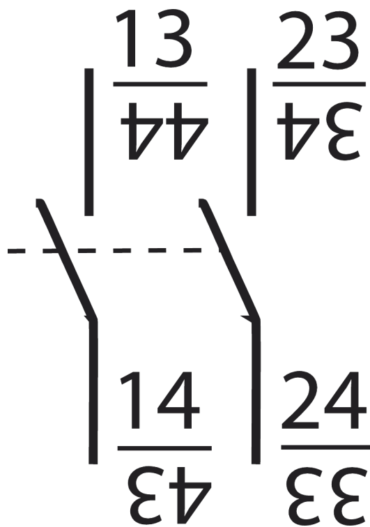
Connection / Wiring Diagram
