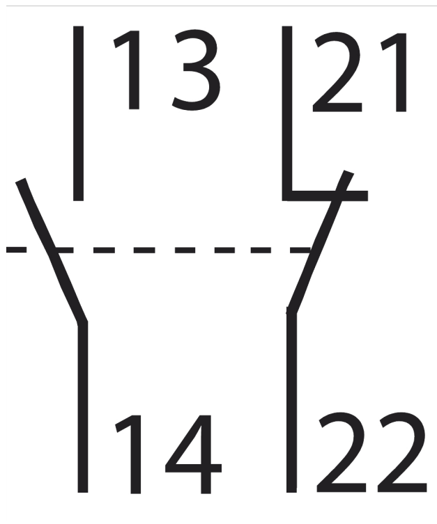
Connection / Wiring Diagram
