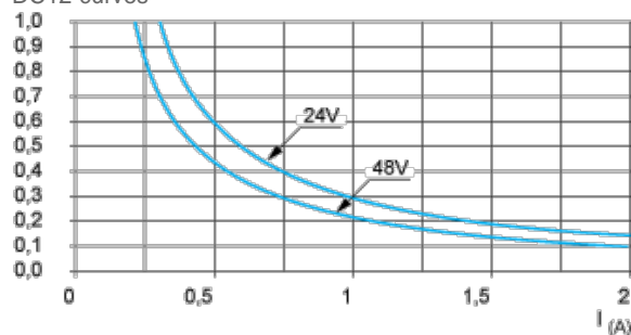
DC12 curves
