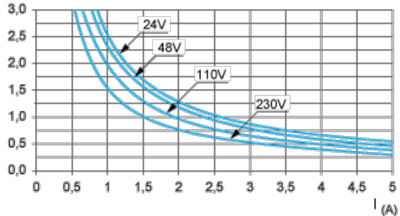
AC12 curves
