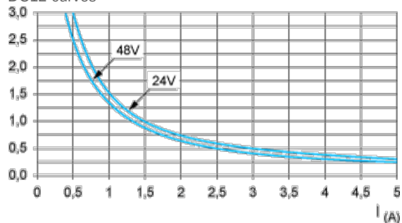
DC12 curves
