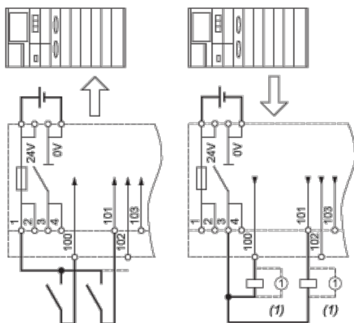
(1) Inductive load
