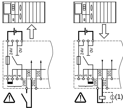
ABE-7H16R20/R21/R23 ABE-7H16R20/R21
