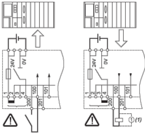
(1) Inductive load
