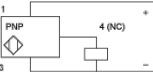
PNP Outputs
