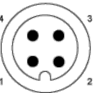
M12 Connector
