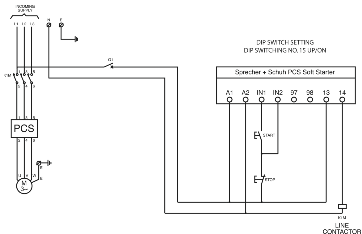
Connection / Wiring Diagram
