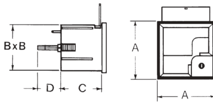
Meter dimensions
