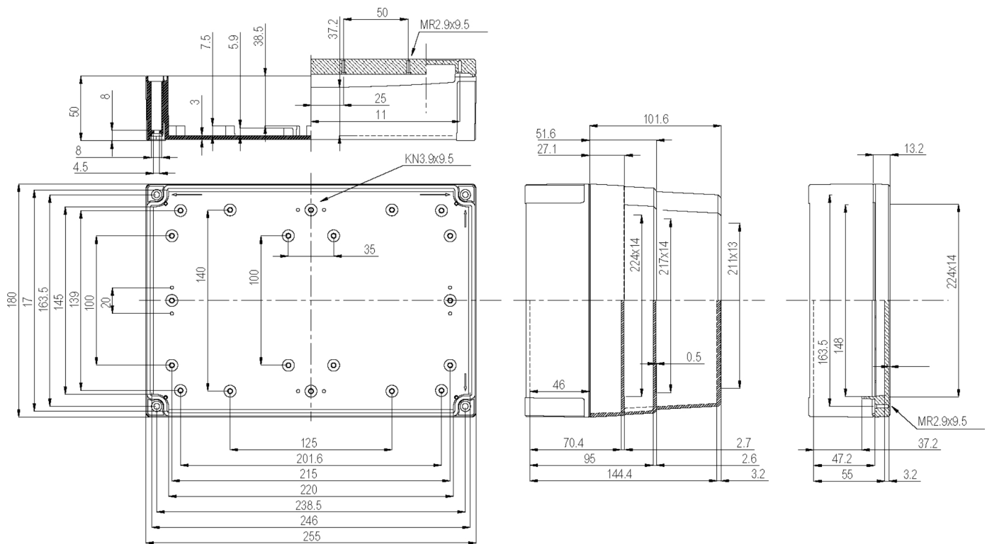
Dimension Diagram
