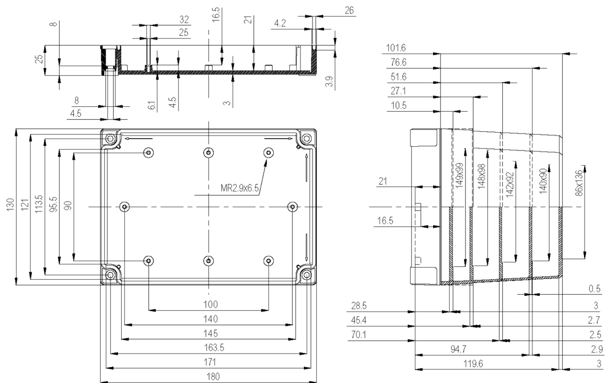
Dimension Diagram
