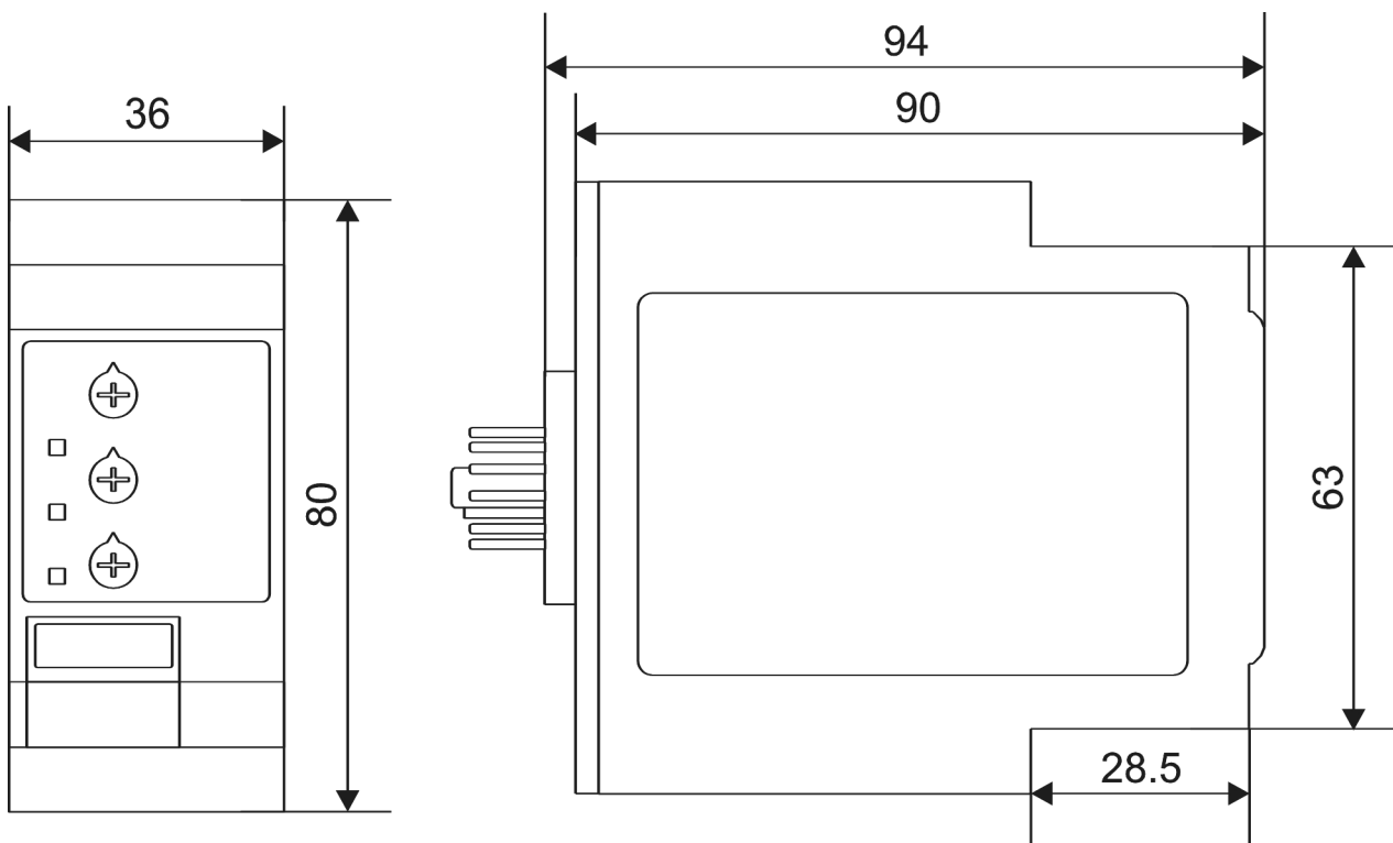
Dimension Diagram
