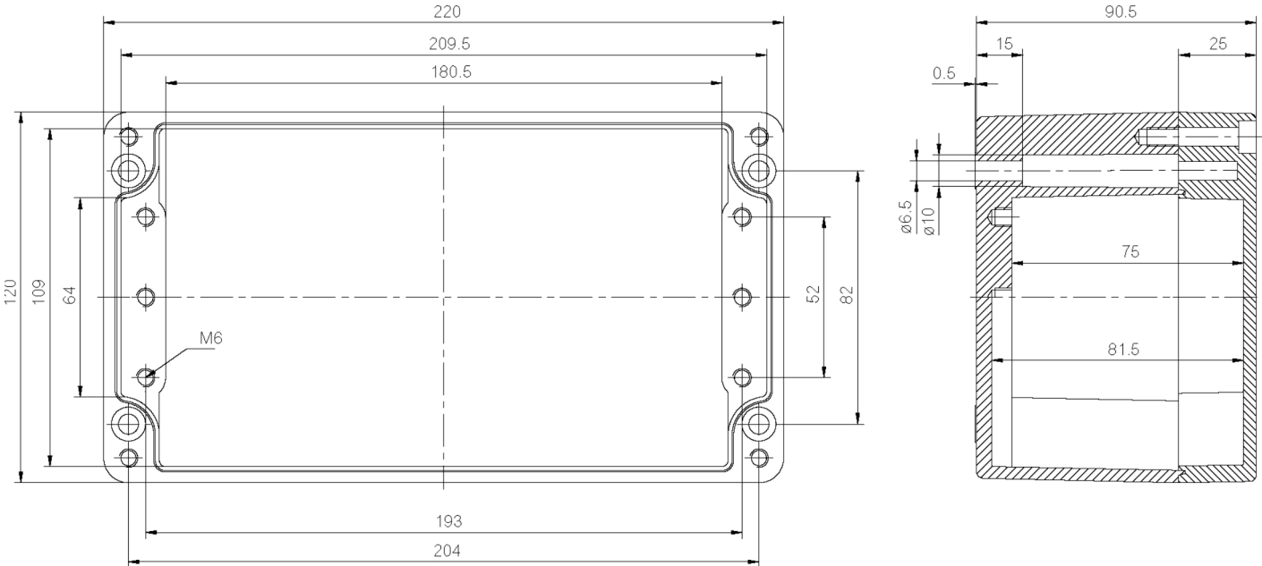
Dimension Diagram
