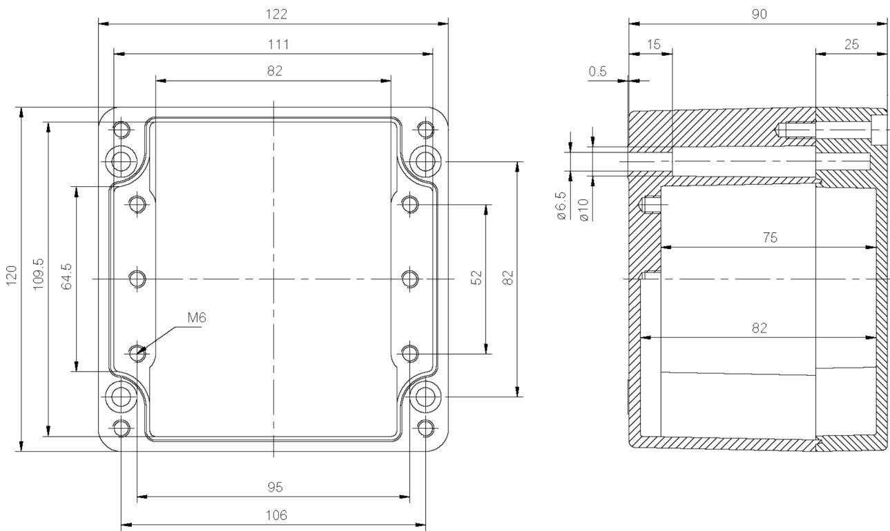
Dimension Diagram
