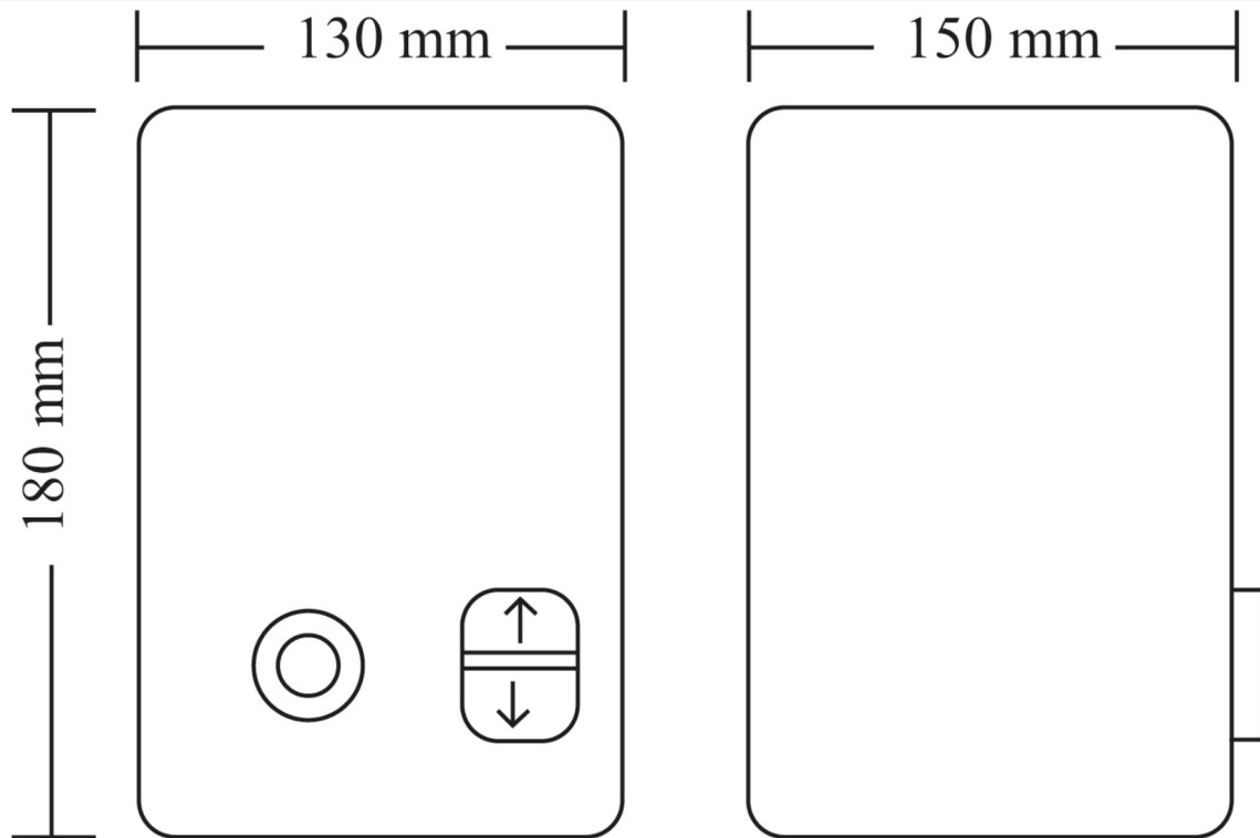
Dimension Diagram
