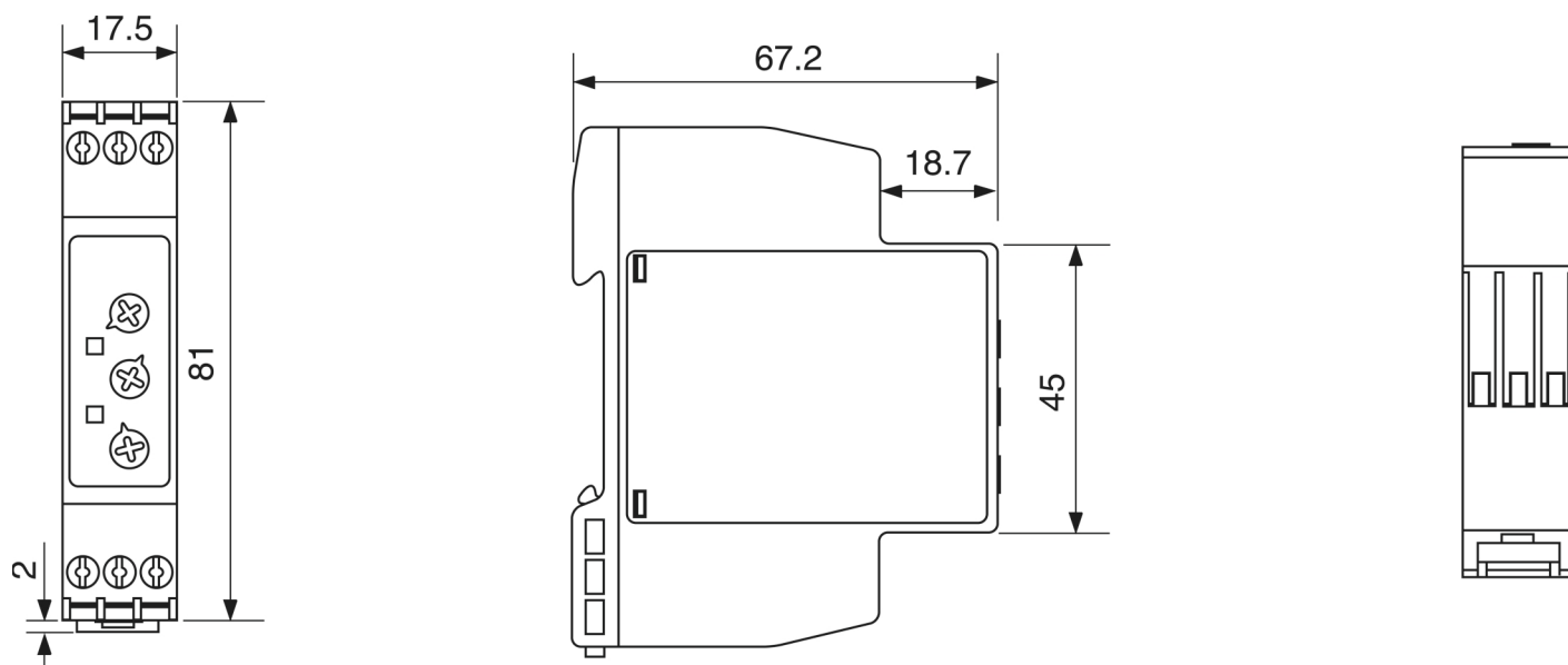
Dimension Diagram
