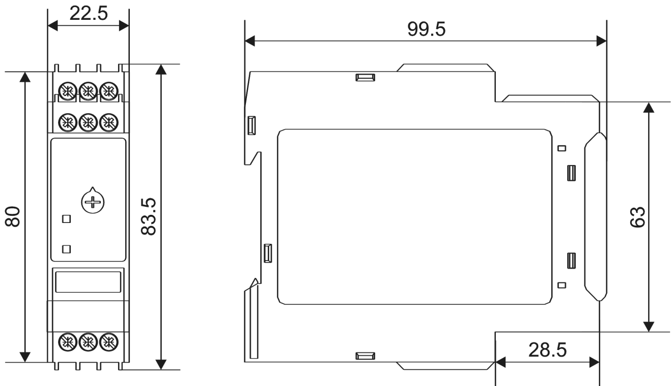
Dimension Diagram
