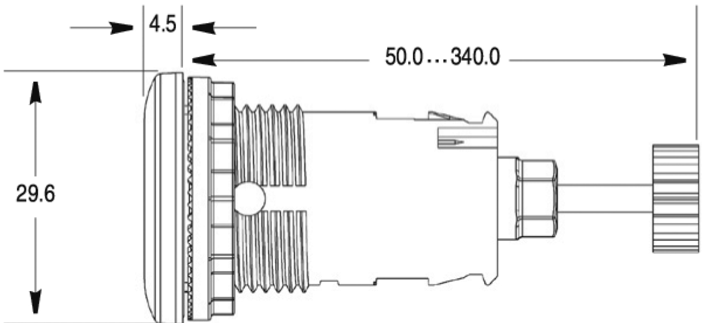
Dimension Diagram
