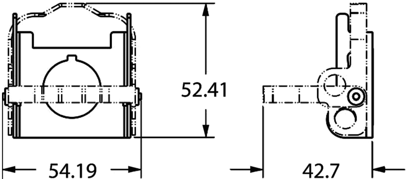
Dimension Diagram
