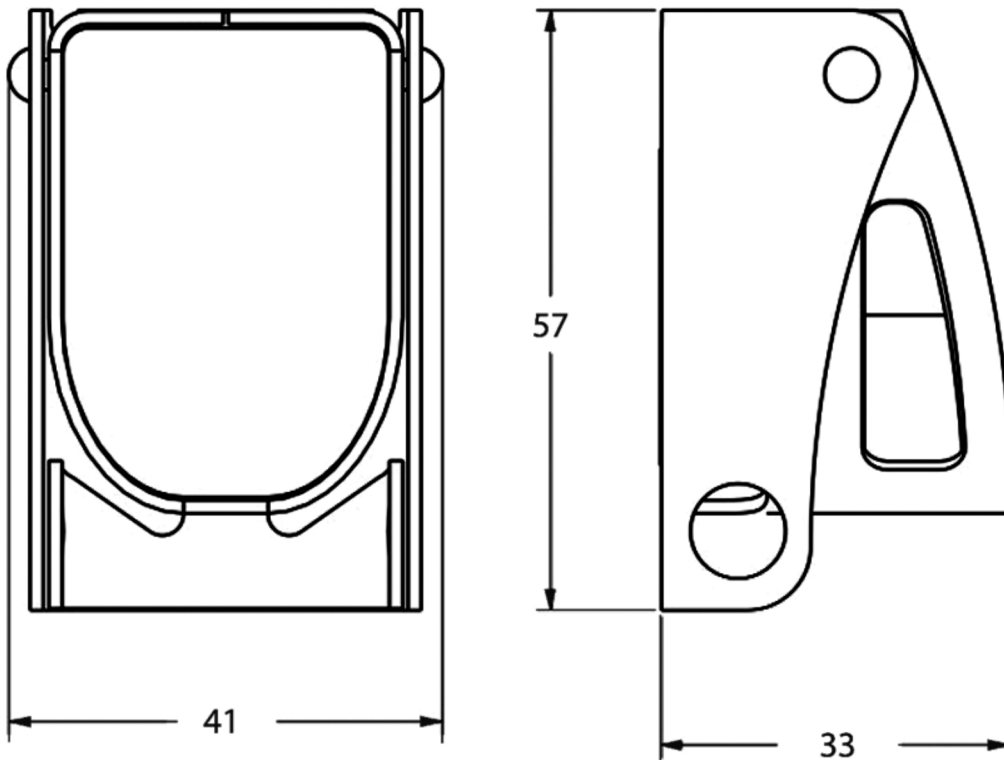
Dimension Diagram
