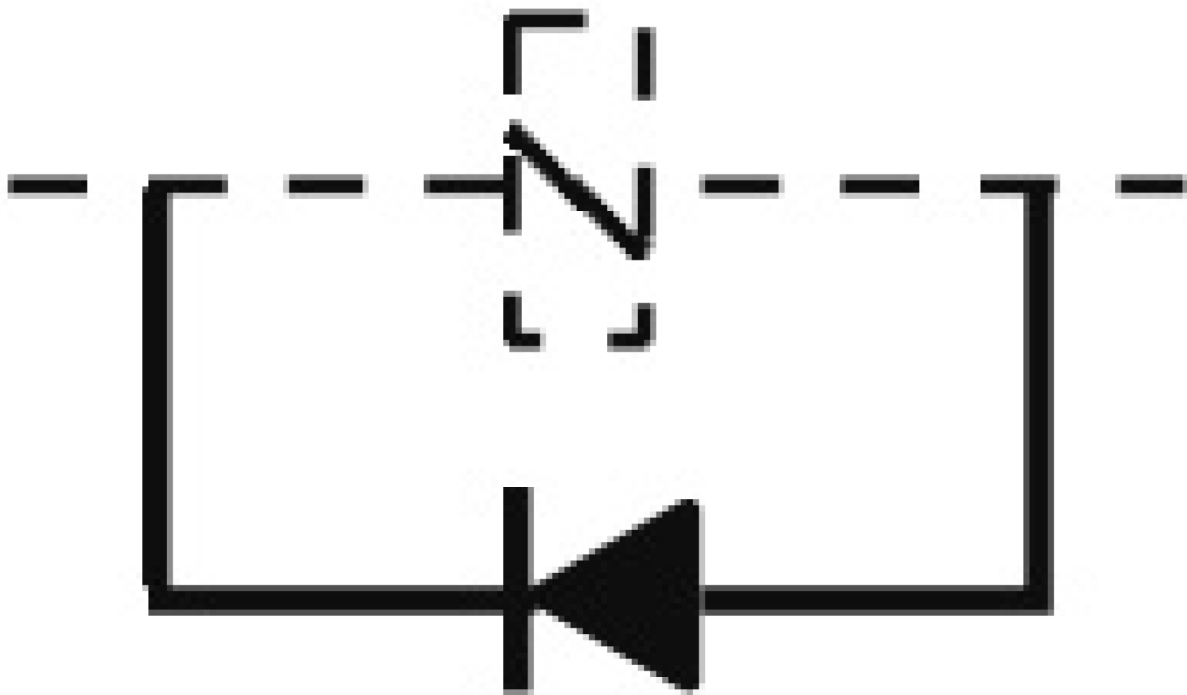
Connection / Wiring Diagram
