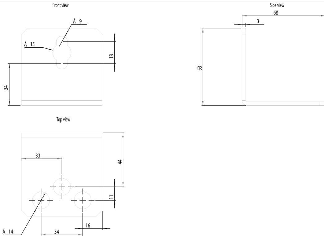
Dimension Diagram
