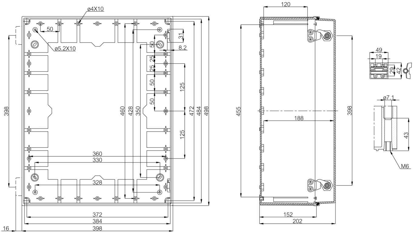
Dimension Diagram
