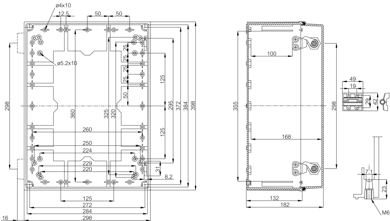
Dimension Diagram
