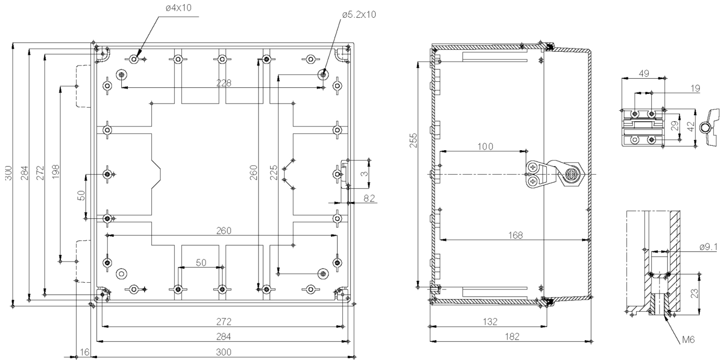
Dimension Diagram
