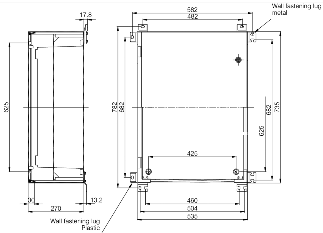
Dimension Diagram
