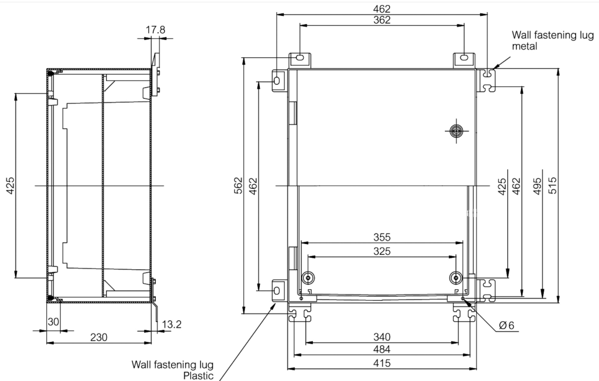
Dimension Diagram
