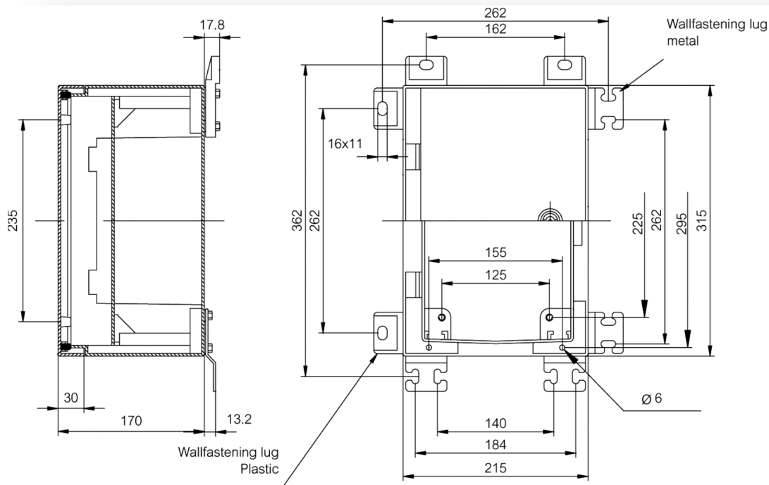
Dimension Diagram
