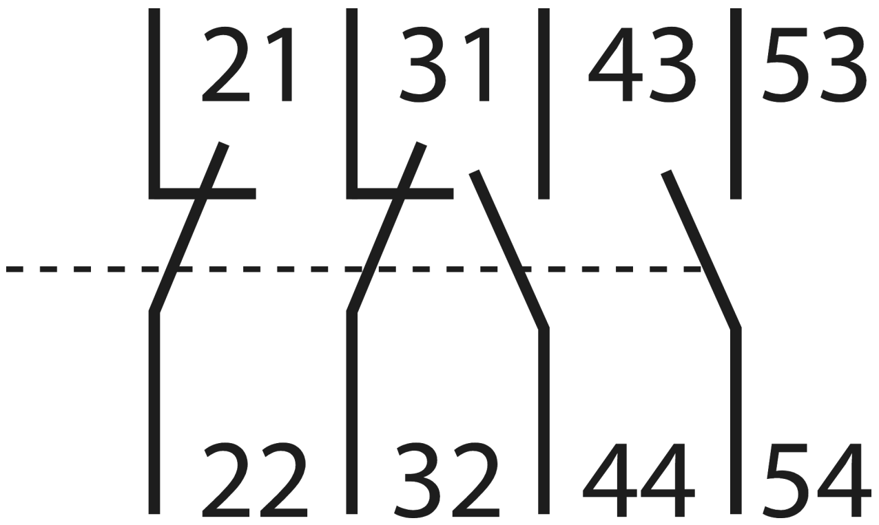
Connection / Wiring Diagram
