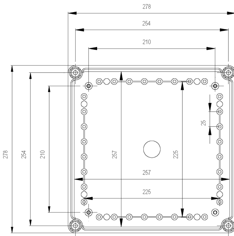
Dimension Diagram
