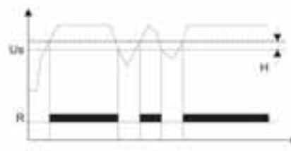
Function E236-US 1.1 and US 2.1
