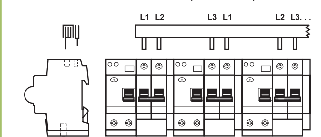
PS 3/28/16 H-DDA 202 T DS 202 + S2C-S/H6R + (DDA 202 + S 202) + S2C-S/H6R ...
