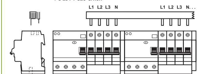
PS 4/36/16 H-DDA 204 T DS 204 (≤ 40 A) + S2C-S/H6R + DS 204 (≤ 40 A) + S2C-S/H6R + DDA 204 (≤ 40 A) + S 204 + S2C-S/H6R + DDA 204 (≤ 40 A) + S 204 + S2C-S/H6R
