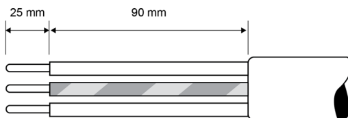
Stripping detail
