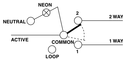
To wire neon permanently "ON"
