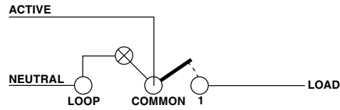
To wire neon permanently "ON"
