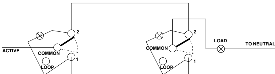
To wire neon "ON" when LOAD "OFF"
