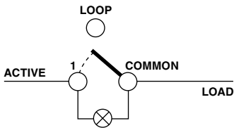
To wire neon "ON" when switch "OFF"
