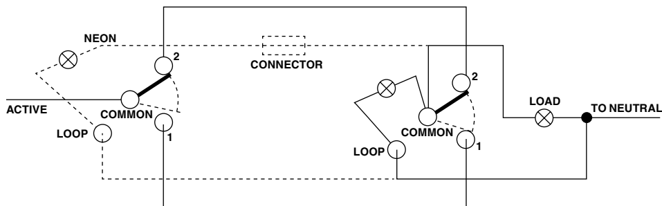
To wire neon "ON" when LOAD "ON"
