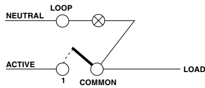
To wire neon "ON" when switch "ON"
