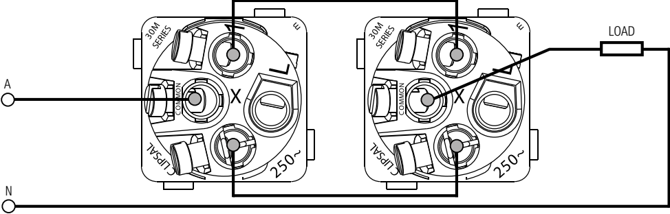
Two-Way Switching
