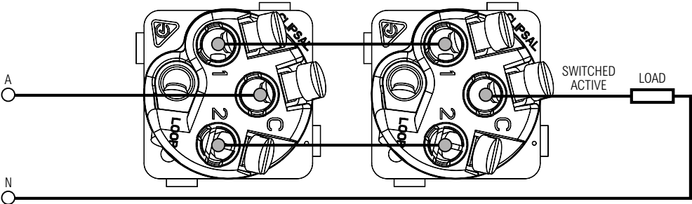
Two-Way Switching
